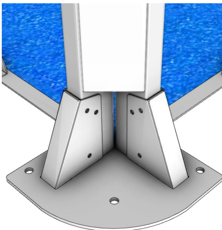
Anchorage plate corner
