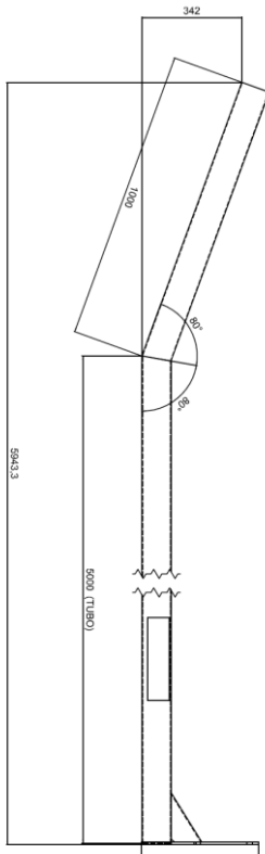
Inclined lighting pillars
