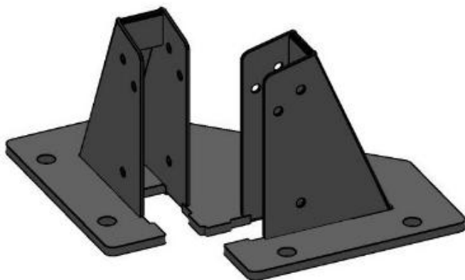
Corner anchor plate P3
