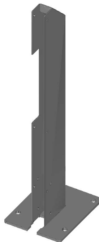
Anchor plate P1B for lighting pillar
